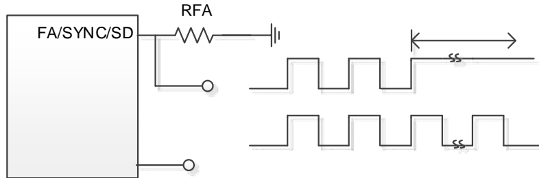
Figure18. Shutdown operation in Frequency Adjust Mode
