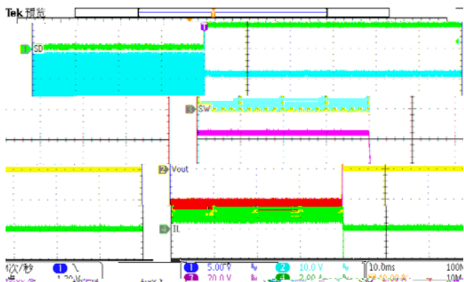
Figure 32. Shutdown entry
