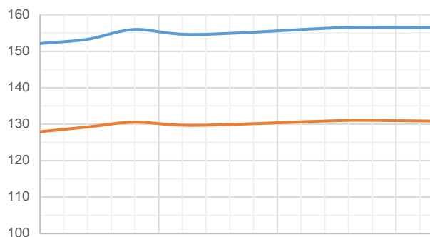
Figure 7. VSENSN vs. Input Voltage
