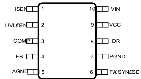
Top View: 10-Lead Plastic MSOP 3mmx3mm
